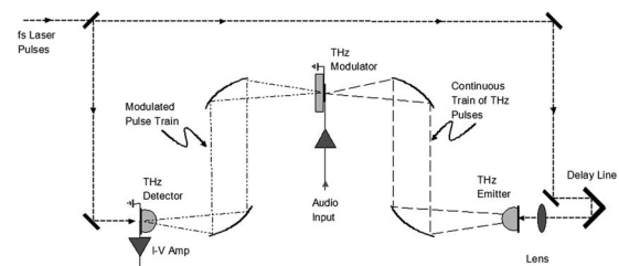
FIG. 13. Experimental setup for analog THz communication link using an external THz modulator (adapted from Ref. 103).
